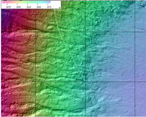
Fig. 3. Gridded Optech scanner data of northwest crater floor at 5 decimeter point spacing with linear filter applied.
