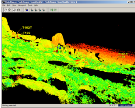
Fig. 2. Leica HDS3000 laser scan of western ejecta field showing Whale Rock in upper center and reflective targets in upper left and middle right.
