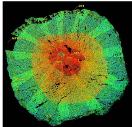
Fig. 1. Optech point cloud scan of crater interior with optical targets marked.
