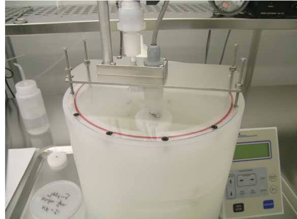
Fig. 1: Genesis Ultra-pure Water Megasonic Wafer Spin Cleaner.
