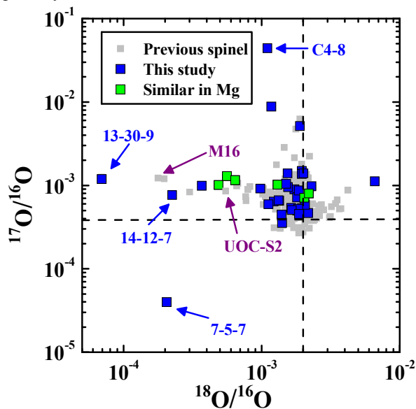
Figure 1. O isotopic ratios of the spinel grains of this study, compared to previous data from references in [11]. The symbol for grain 13-30-9 completely covers the spot where OC2 [3] would plot. The grains plotted as green squares correspond to the grains circled in Fig. 2.
