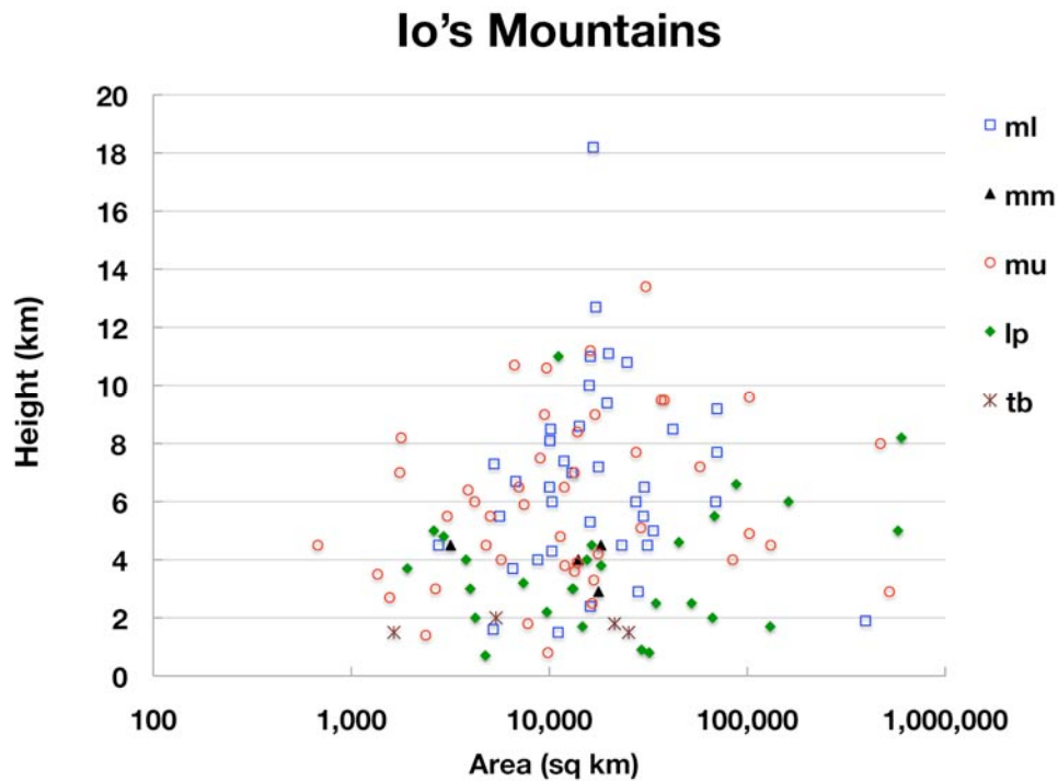
Figure 1. Plot of area-height relationships of Io's mountains. Mottled mountains (mm) are generally less high than lineated mountains (ml), consistent with their degradational formation. Undivided mountains (mu) are widely distributed, as lack of resolution inhibits better characterization. Tholi (volcanic mountains, tb) are of low relief, consistent with formation from low-viscosity lavas. Layered plains are mostly <6 km high, consistent with highly degraded mountains, grading into eroded plains (i.e., 'resurfacing' by mass wasting, a minor process on Io).
