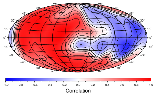
Fig. 1 Map of localized correlation value for L_{win} = 5 at harmonic degree of 15.
