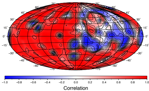
Fig. 2 Map of localized correlation value for L_{win} = 17 at harmonic degree of 30.
