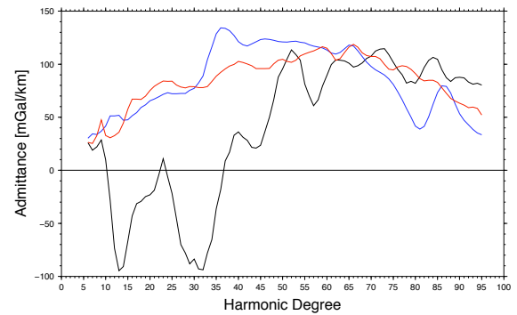
Fig. 4 Localized admittance spectra of SPA (red; window center = 180, -56), FHT (blue; window center = 180, 0) and near-side (black; window center = 0, 0) ( L_{win} = 5 ).
