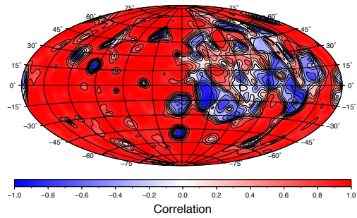
Fig. 3 Map of localized correlation value for L_{win} = 26 at harmonic degree of 40.
