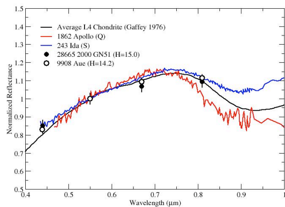
Figure 1: Colors of two objects observed at KPNO in Dec 2008, compared to two asteroids and an ordinary chondrite meteorite [6,15]. Although the wavelength coverage for these data is not optimal for covering the 1- \mu\text{m} band, the observed objects show spectra consistent with the average L4 chondrite. The asteroid data are normalized to the V band, at 0.55 \mu\text{m} .
