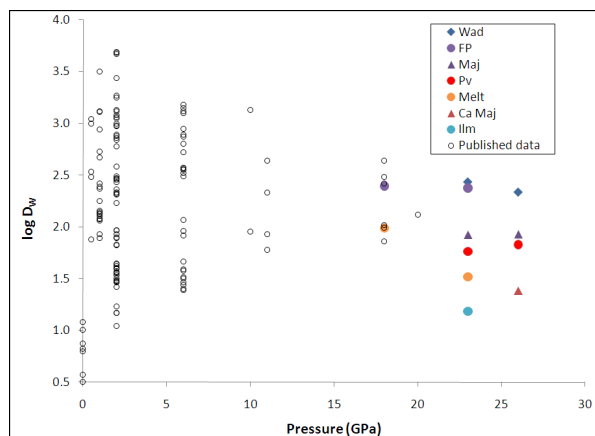
Figure 2. Plot of \log D vs. pressure for W. D_W values from our experiments are metal/mineral coefficients. Uncertainties on D_W range from 8% to 24%. Published data are shown for comparison.
