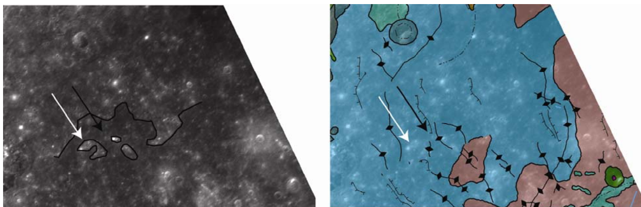
Figure 2. MESSENGER high-resolution narrow angle camera data (left) showing intra-ejecta dark plains (black arrow) interfingering hummocky ejecta (white arrow) within the Odin Formation (right, blue unit, from Schaber and McCauley [1980]).
