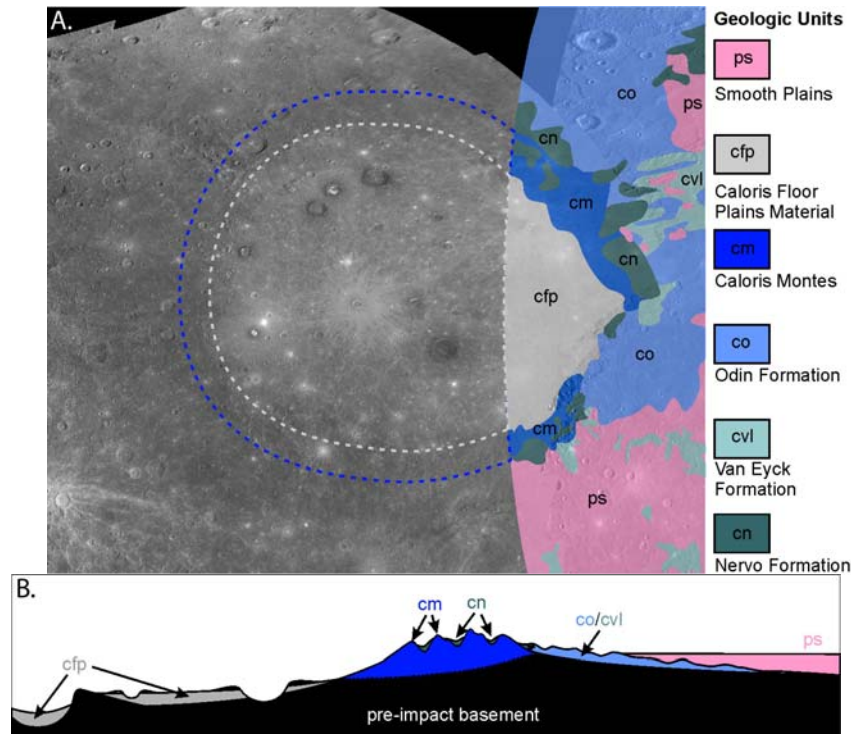
Figure 1. A) Mosaic of Mariner 10 (colorized, right side) and MESSENGER (left) high-resolution narrow angle camera data for the Caloris basin. Overlain on the Mariner 10 data are sketch geologic units after Schaber and McCauley [1980] and Guest and Greeley [1983] (crater and ejecta-related materials not included). Dashed lines illustrate the approximate extension of the Caloris Floor Plains Material unit (grey) and the Caloris Montes basin rim unit (blue). B) Schematic geologic cross-section from the Caloris basin center (left edge) and outward. Odin (co) and Van Eyck (cvl) Formations are combined for simplicity.
