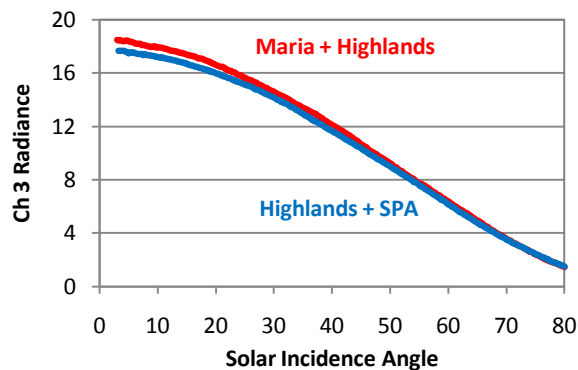
Figure 2: Radiance vs. Solar Incidence Angle. Highlands + SPA terrain is defined as mostly farside longitudes between 100E and 75W, while maria + highlands terrain is mostly nearside between 75W and 100E.
