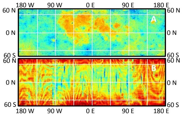
Figure 1: Diviner Preliminary CF Value and Fractional Coverage Maps. 1A: 8 pdd CF values scaled 7.8 (blue) to 8.55 (red). 1B: 1 ppd Fractional coverage scaled 0 (blue) to 1 (red). Most coverage gores were caused by LRO rolls for targeted observations.
