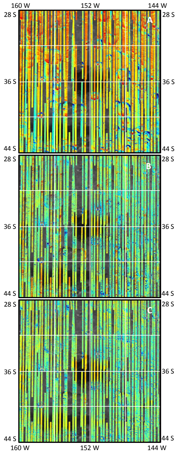
Figure 3: Apollo Basin Brightness Temperature and CF Value Maps. 3A: 8 \mu\text{m} brightness temperature, scaled 300 K (blue) to 400 K (red). 3B: CF values from standard radiance, scaled 7.8 (blue) to 8.55 \mu\text{m} (red). 3C: CF values from highlands + SPA normalized radiance. Diviner strips are 128 ppd. The basemap is Clementine 750 nm albedo.
