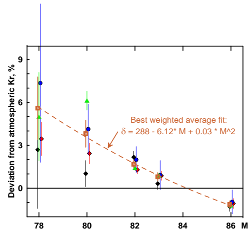
Figure 2. Deviations of calculated solar wind composition from analyses of Genesis Al-collectors (four different sets of measurements) are consistent. Symbol and color notations are the same as in Fig. 2. Bold brown squares are weighted average values best fitted by slightly unlinear curve, which is probably not statistically significant.
