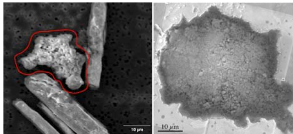
Figure 2. Secondary electron images of particle 2-7-9.009 on the Pt-coated Nuclepore filter (left) and pressed into Au foil (right).
