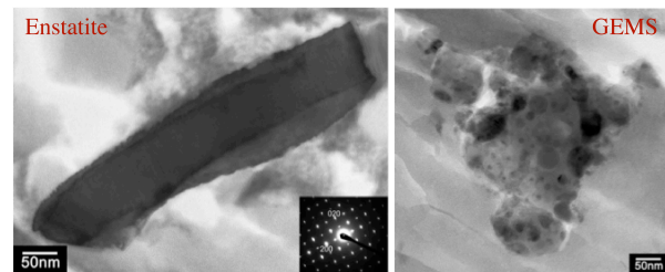
Figure 1. Enstatite platelet (left) and GEMS (right) in TT54B397.
