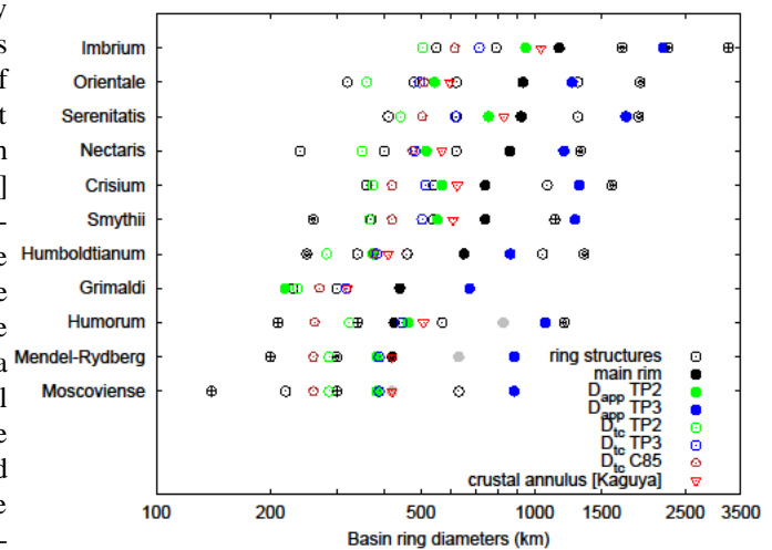
Figure 2. Structural features for a suite of 11 lunar basins. Data includes: ring diameters [24] (open black circles represent definite ring structures; partially filled circles represent uncertain ring structures), main rim diameter estimates [2] (black circles), alternative basin rim diameter estimates [25] (gray circles), transient crater diameter estimates from [26] (C85) and this study, and crustal annulus diameter estimates (Kaguya data). Data from this study for thermal profiles TP2 (green circles) and TP3 (blue circles) plot either side of scaling estimates and observations for a given basin feature. Dtc is the transient crater diameter; Dapp is the apparent basin rim diameter.
