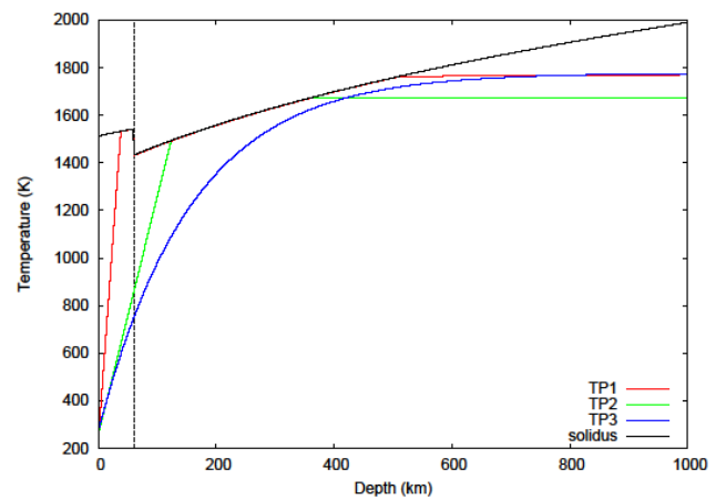
Figure 1. The three temperature profiles investigated. TP1: near-surface gradient of 34 K/km; ~1770 K deep mantle temperature. TP2: near-surface thermal gradient of 10 K/km; ~1660 K deep mantle temperature. The temperature profiles are bound by the solidus so temperatures never exceed the ambient melt temperature. TP3 is modified from [18] and estimates a 0.5 Gy old Moon. Dotted line is crust/mantle boundary (60 km depth).
