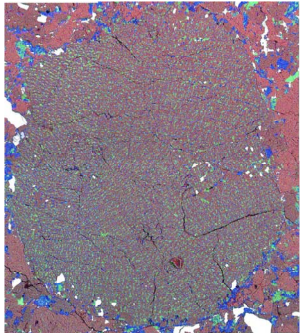
Figure 3 – Elemental Map of Melt Clast in PRE 95400. Blue = Aluminum, Red = Magnesium, and Green = Calcium (FOV = 600 microns across)
