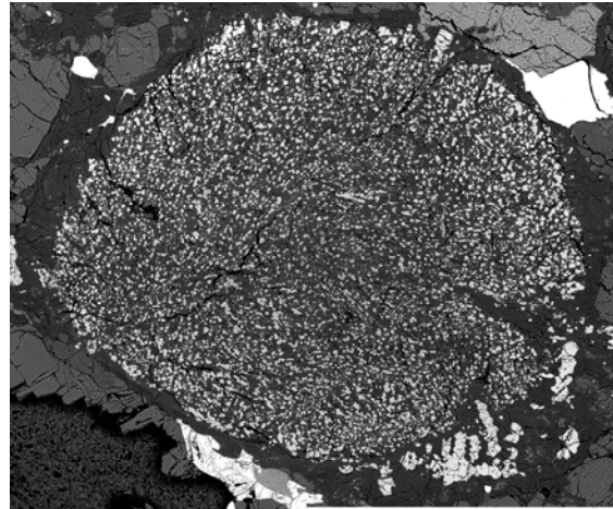
Figure 2 – Backscattered electron image of a melt clast found in MET 01002. (FOV = 600 microns across).
