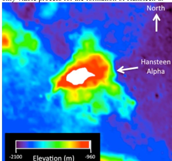
Figure 2. Hansteen Alpha DEM generated from the GLD100.
