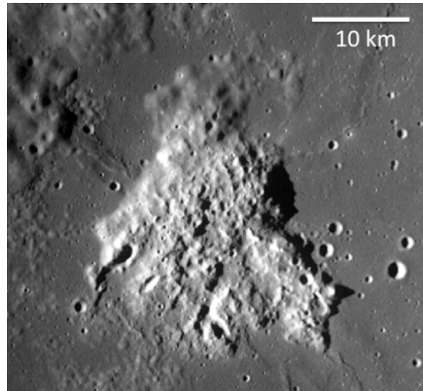
Figure 1. Portion of WAC frame M117826631ME
