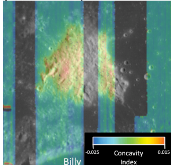
Figure 3. Diviner concavity map overlaid on WAC frame
