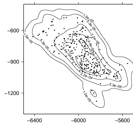
Figure 1: Spatial density distribution of vents on Syria Planum. In both figures, contours represent the 25 th , 50 th , 75 th , 95 th , and 99 th percentiles of vent density; black circles represent volcanic vents; north is up; eastings and northings are given in Transverse Mercator kilometers.
