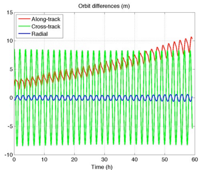
Figure 5. Orbit differences in short LRO arcs induced by the use of ‘direct altimetry’ measurements during the POD convergence.
