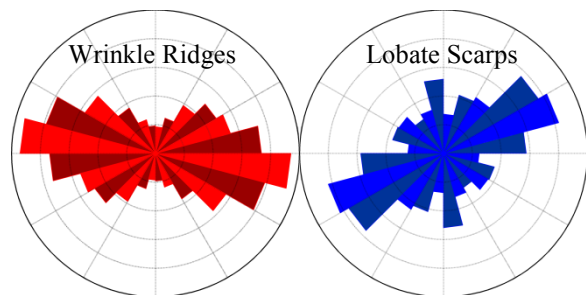
Fig. 2: Length-weighted distribution of mapped Frigoris tectonic landform orientations.
