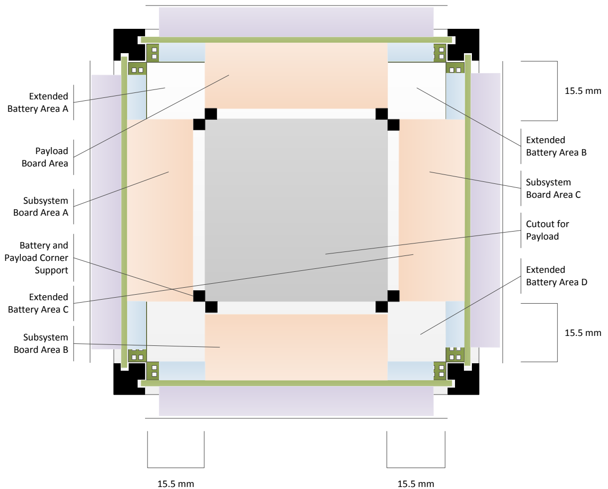
Figure 1. Open Prototype for Educational NanoSats Spacecraft Design [5]
