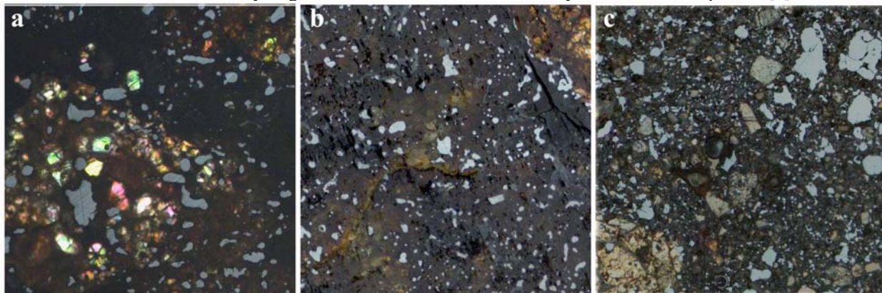
Figure 2. A 1 mm 2 window of three of the chondrites discussed here exhibiting increasing amounts of metal in this Zeiss petrographic microscope reflectance image: a) GRA 95229, b) EET 92159, and c) PCA 91467.
