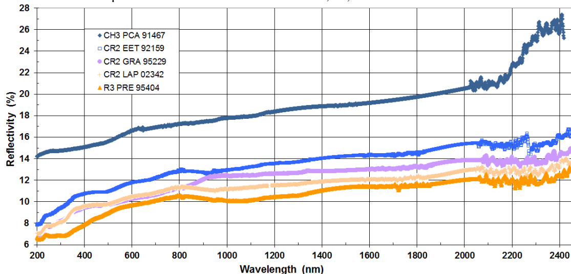
Figure 1. UV-NIR spectra of CH, CR, and R carbonaceous chondrites. A higher abundance in pyroxene-rich chondrules in the CHs is the likely origin of the NIR increase in reflectivity from 2.200 nm upwards [4].
