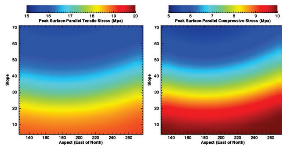
Figure 4. Effects of slope and aspect on peak surface-parallel extensional (left) and compressive (right) stresses experienced by water ice under 5mm of dust.
