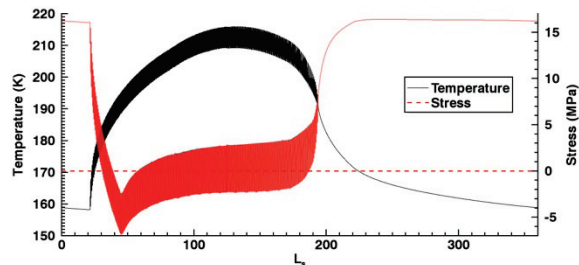
Figure 3. Example thermal behavior of water ice buried by 5mm of dust with a 45^{\circ} SW-facing slope (black). Surface-parallel stress (positive indicates tension) is in red (right axis).
