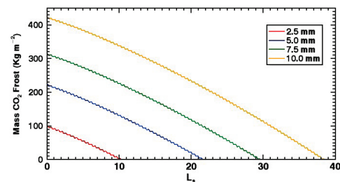
Figure 2. \text{CO}_2 frost on a 45^\circ SW-facing slope of water ice with dust covering of different thicknesses.
