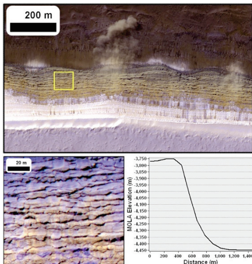
Figure 1. HiRISE image (PSP_007338_2640, L_s 34) of 70^\circ scarp (MOLA topography at bottom right) at 84^\circ\text{N} 235^\circ\text{E} with avalanche in progress [10]. Yellow box shows location of scarp texture in bottom left.
