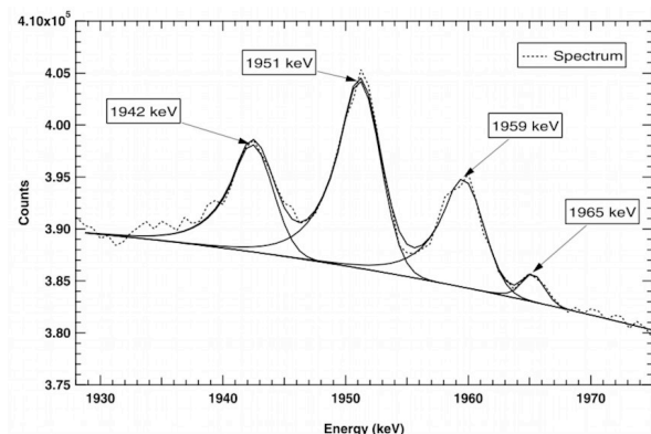
Figure 2. Gamma ray spectrometers are very sensitive to chlorine! The Mars Odyssey GRS measured Cl abundance was 0.49\% \pm 0.3\% . The GRS spectrum above shows strong Cl and Ca lines, demonstrating a gamma ray spectrometer's ability to detect salts. The peaks are from \text{Ca}(n, \gamma) at 1942 keV and two \text{Cl}(n, \gamma) lines at 1951 and 1959 keV. [6]
