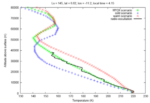
Figure 3: A typical temperature profile obtained by MGS radio occultation in May 1999, compared to profiles predicted by the MCD at the same time and location using various dust scenarios. Profiles obtained using the MY24 scenario are usually close to the MGS observations, whereas those obtained using the warm (dusty) and cold (clear sky) scenarios are typically respectively warmer and colder.
