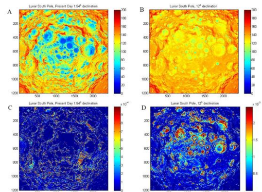
Figure 1: (A) Mean annual temperature in the current ( 1.54^\circ tilt) lunar south polar region (stretched 0-200K), (B) Mean annual temperatures at 12^\circ tilt, (C) Modeled ice mass ( \text{kg m}^{-2} \text{yr}^{-1} ) gained at 1.54^\circ assuming simple model [8], (D) Modeled ice mass ( \text{kg m}^{-2} \text{yr}^{-1} ) gained at 12^\circ .
