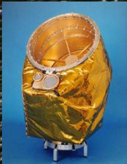
Cassini's Cosmic Dust Analyzer
