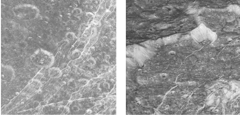
Fractures on Dione at pixel scales: 230 m (left) and 23 m (right)
