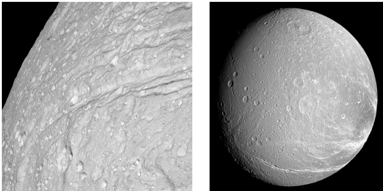
Ithaca Chasma, Tethys (left) and fractures on Dione (right)
