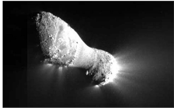
Comet Hartley 2, NASA EPOXI
