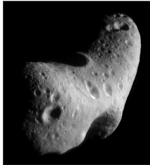
Eros, NASA NEAR Shoemaker
